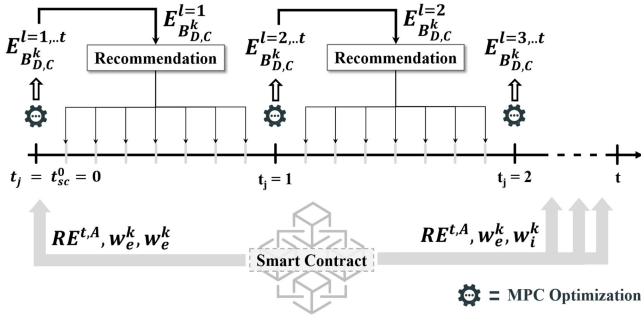
Fig. 3. MPC process with smart contract communication.
